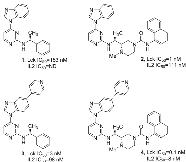
Figure 1. Disubstituted pyrimidines as inhibitors of Lck.
